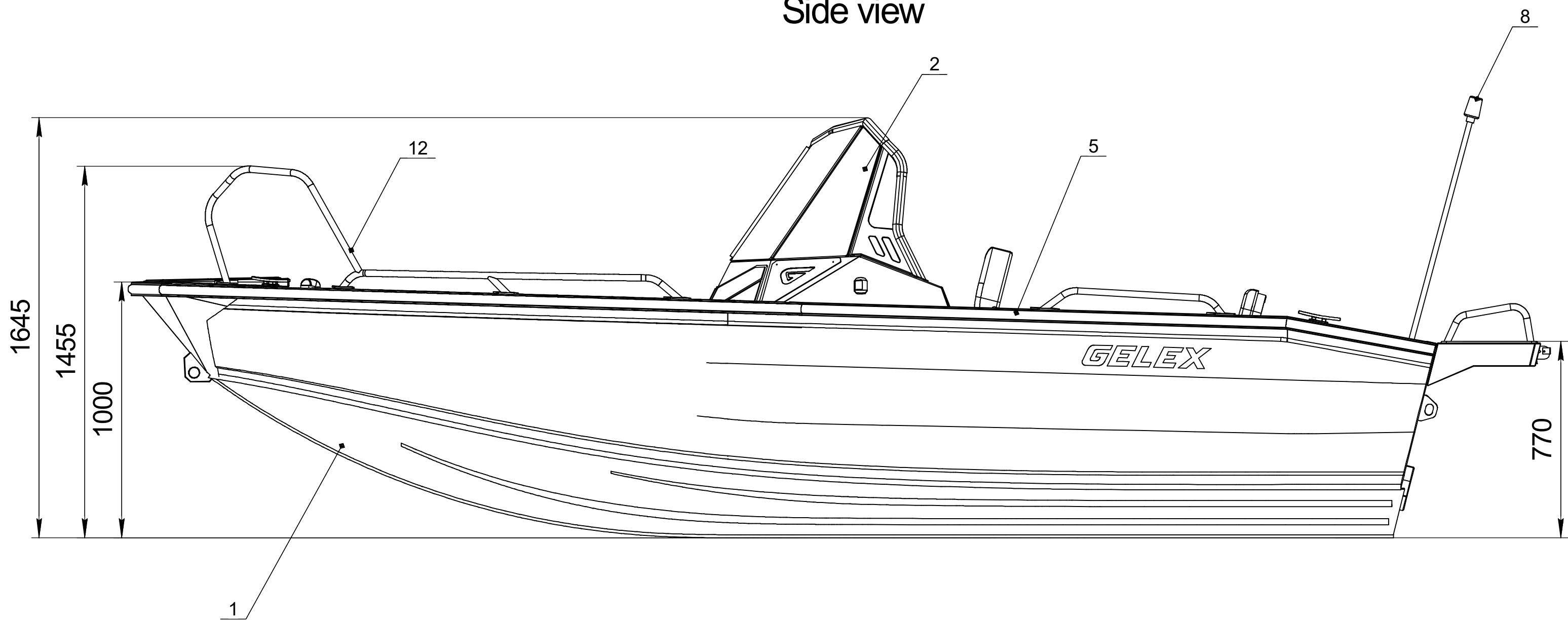
Side view
