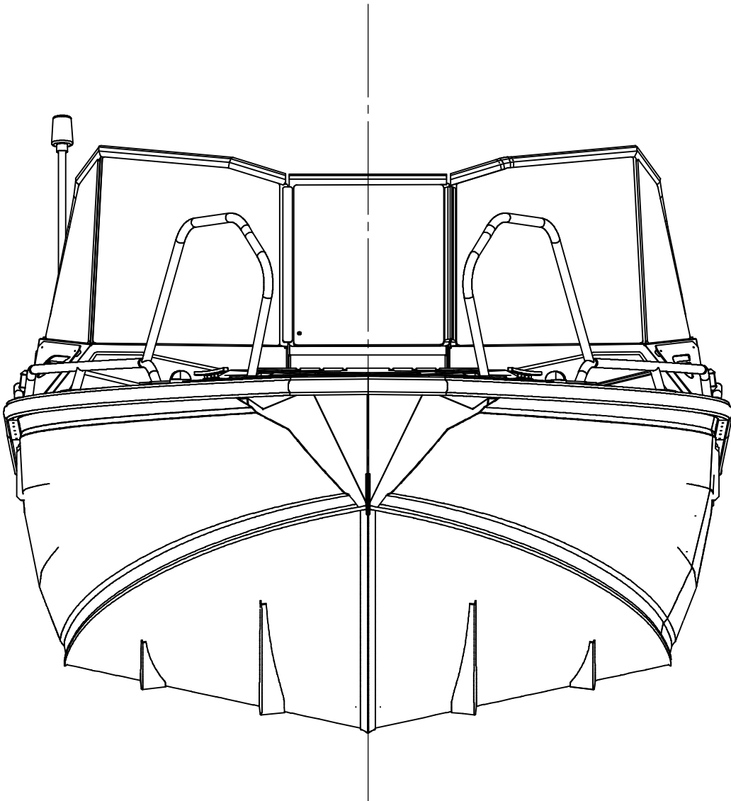
Bow view
