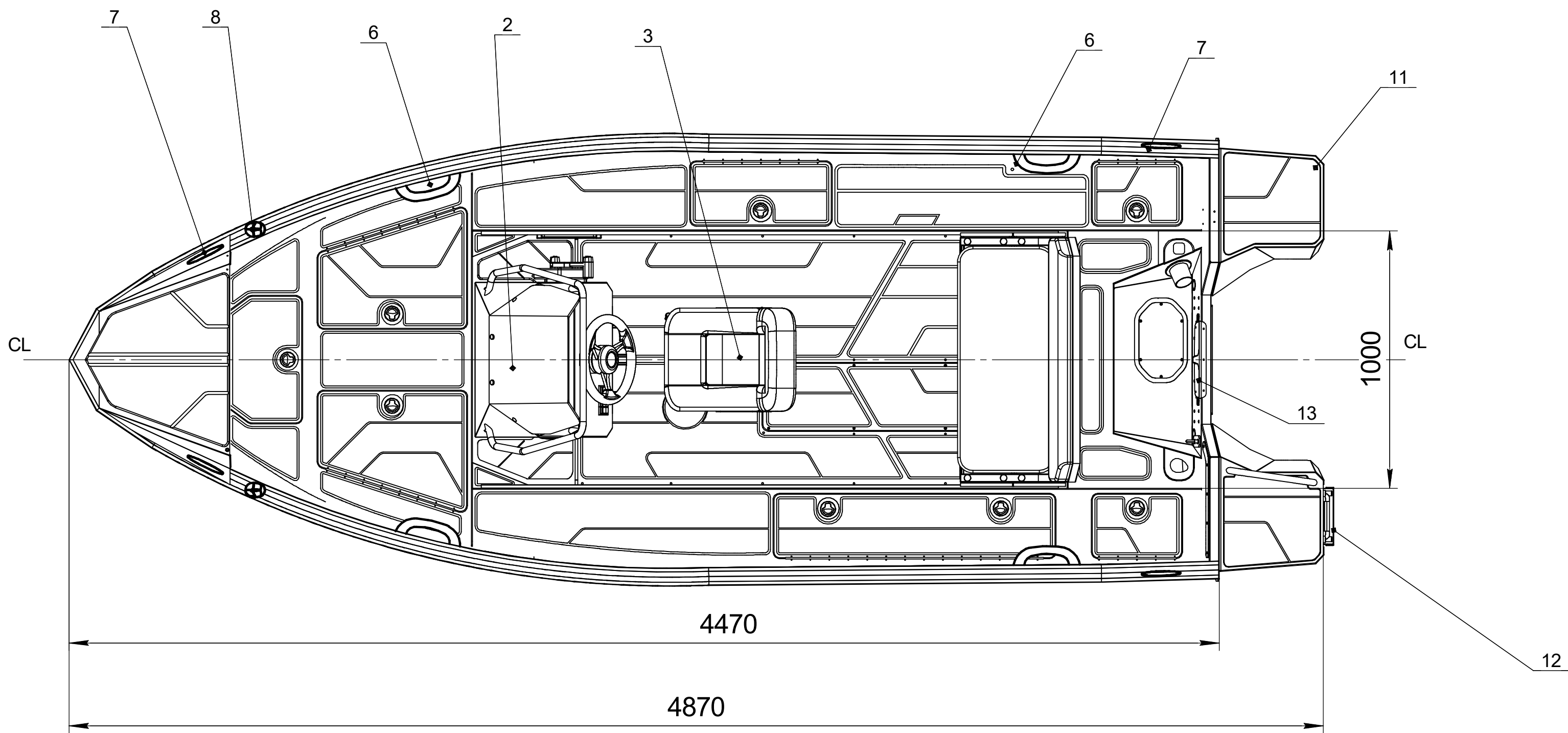
Top view
